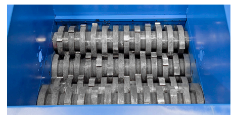
Shredder Chamber
